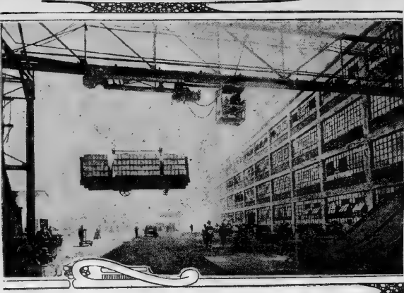
Thousands of tons of freight are carried each year on the monorail trolley in the big Ford factory. This trolley system of 6,885 feet of overhead rail does away almost entirely with hand-trucking and effects a big saving both of time and money.
